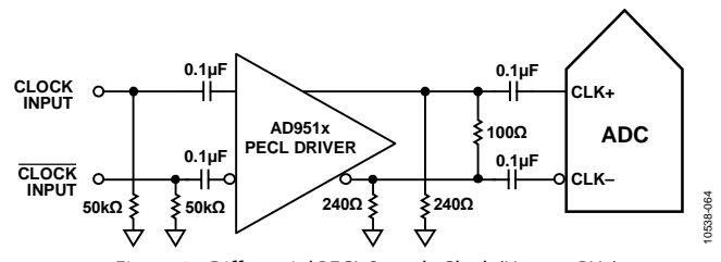
Figure 64. Differential PECL Sample Clock (Up to 1 GHz)
